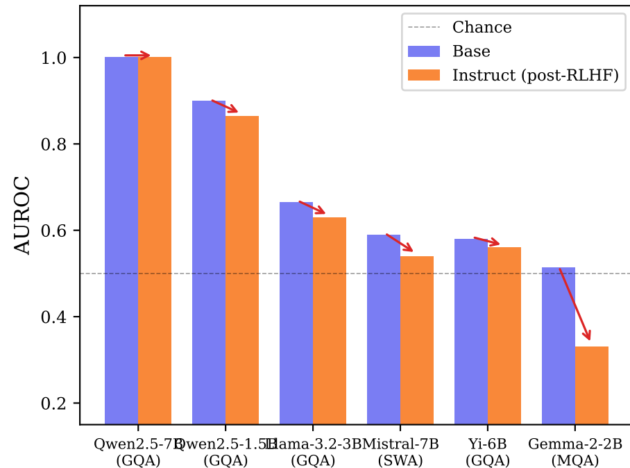
RLHF attenuation by model family
