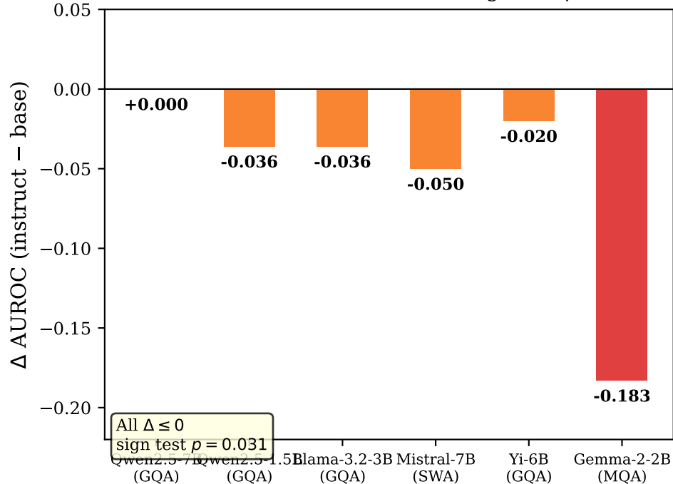
RLHF \Delta (monotone with baseline, sign test p = 0.031 )
