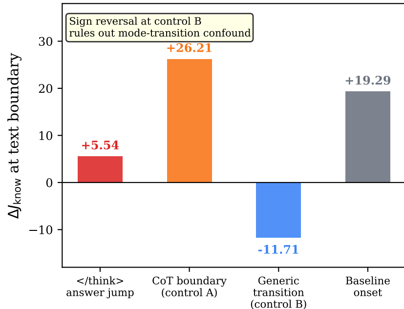
Answer jump at </think> boundary (DeepSeek-R1-Distill)
