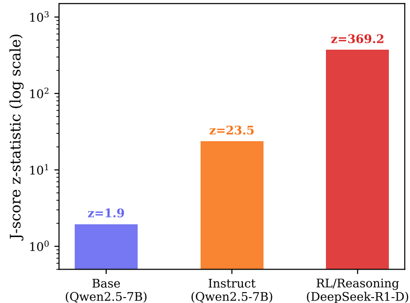
Commitment sharpness by training regime
