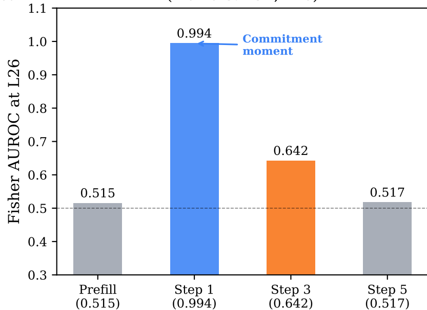
Phase transition at generation step 1 (Llama-3.2-3B, L26)
