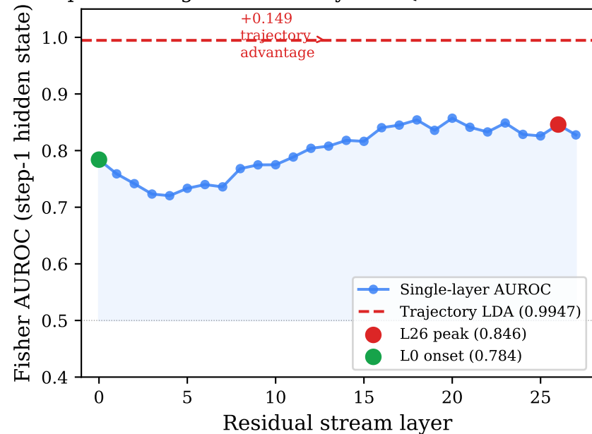
Epistemic signal at each layer — Qwen2.5-7B-Instruct
