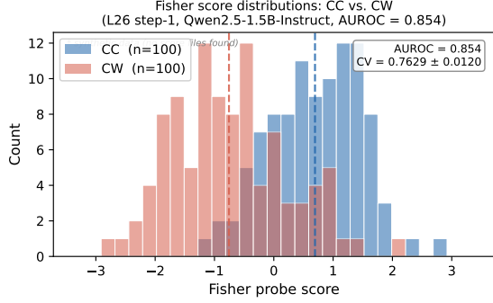
Figure 1: Fisher+PCA64 score distributions for CC (confident-correct) and CW (confident-wrong) items. AUROC = 0.854 despite both classes having identical low output entropy by construction. The separation is genuinely hidden-state-specific.
