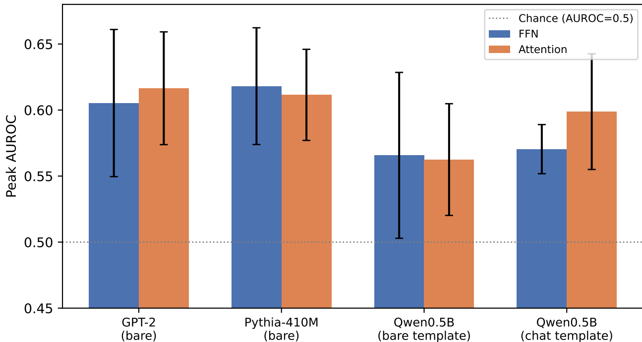
FFN vs. Attention peak AUROC: consistently close, and the only architecture with a clear leader reverses under template correction
