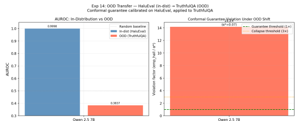
Figure 8: OOD transfer collapse (Exp. 14): Qwen 2.5 7B probe trained on HaluEval (AUROC = 0.9998) and applied to TruthfulQA (AUROC = 0.384, 14.2\times conformal violation). The AUROC drop of 0.616 is the largest observed across all experiments. A third architecture, GPT-2 Medium, was added post-review (§7.2: in-dist 0.9859 \rightarrow OOD 0.5562, 14.1\times violation). It is not re-plotted here; it shows the identical qualitative collapse pattern.
