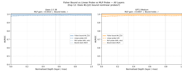
Figure 3: Fisher bound \Phi(\sqrt{J/2}) (solid), linear probe AUROC (dashed), and MLP probe AUROC (dotted) at every layer. The shaded region is the bound slack. The bound is never violated by the MLP probe on either model.
