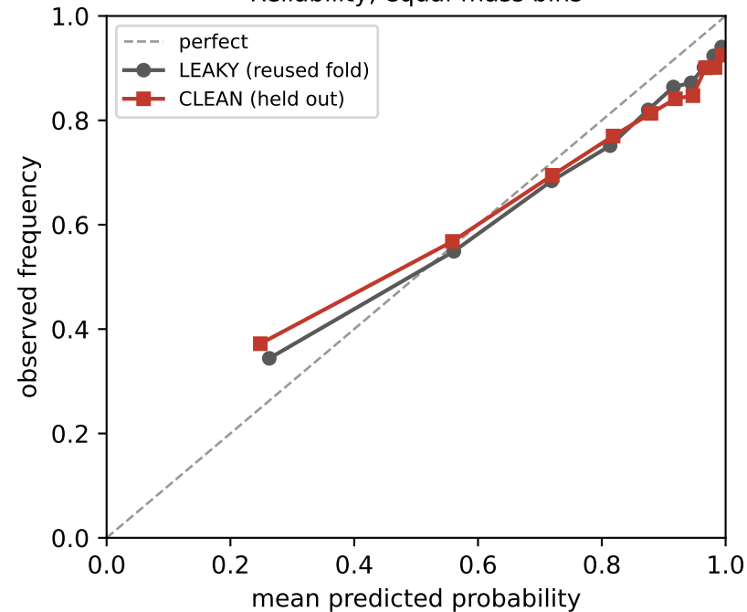
Reliability, equal-mass bins
