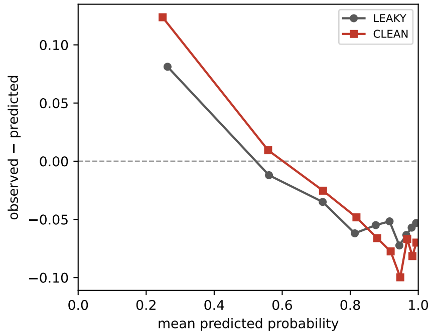
Deviation from calibration
