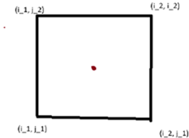
Figure 1: two dimensional interpolation done with flat extrapolation
