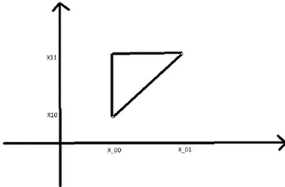
Figure 2: two dimensional interpolation done with flat extrapolation
