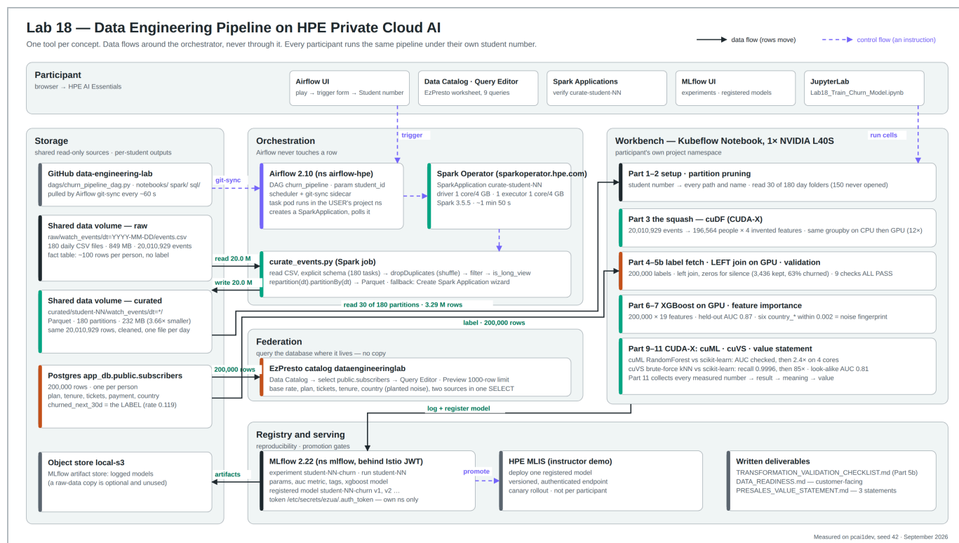
Figure 1. Lab architecture on HPE Private Cloud AI. Solid arrows carry rows; dashed arrows carry instructions. Airflow sits on a dashed path only.
