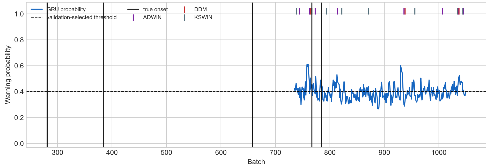
Drift timeline — insects_abrupt_balanced
