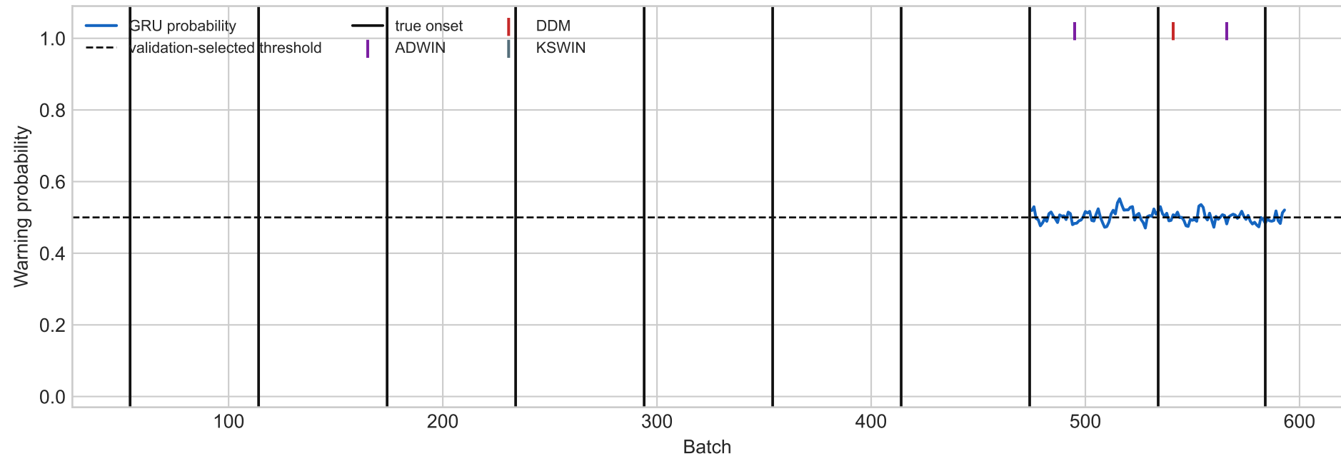
Drift timeline — synth_sea_gradual
