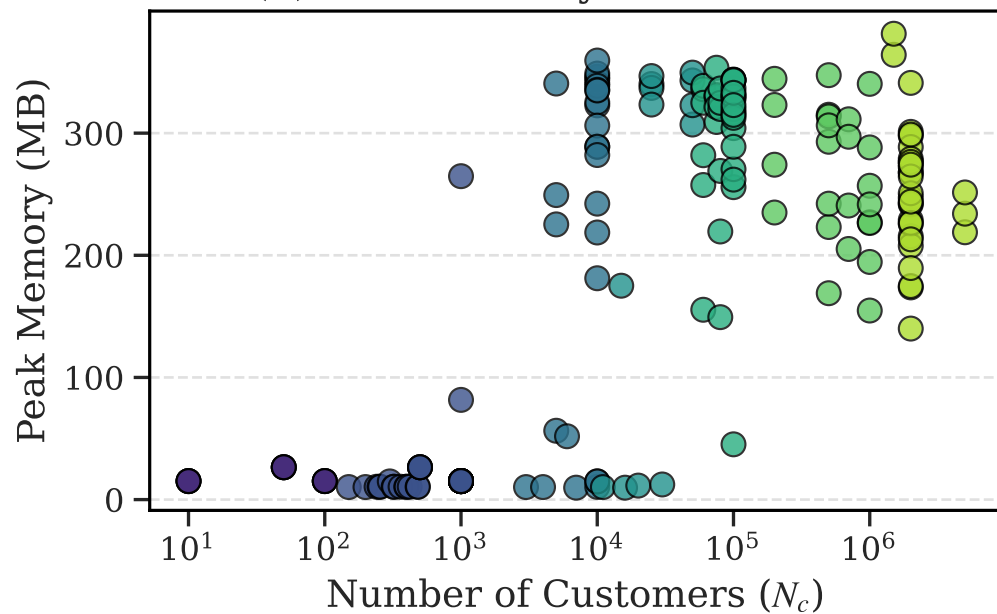
(b) Peak Memory vs. Customers
