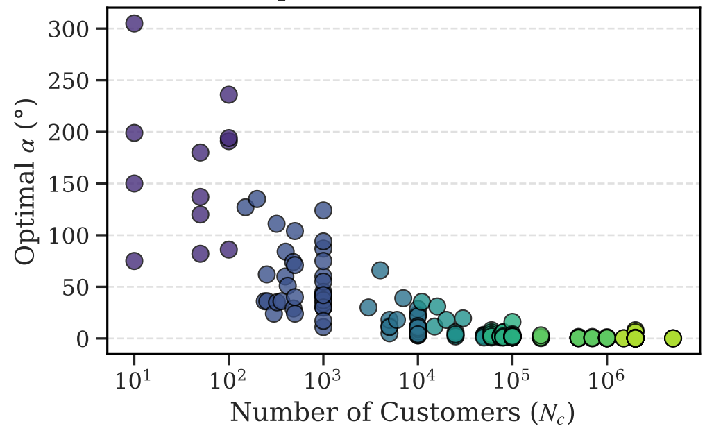
(c) Optimal \alpha vs. Customers
