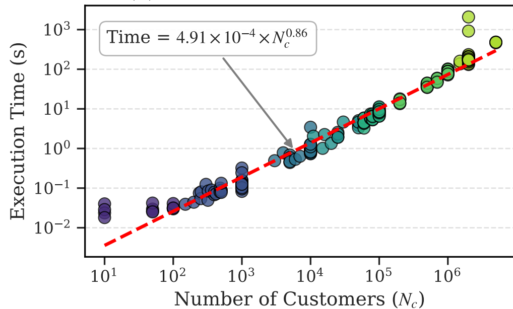
(a) Execution Time vs. Customers
