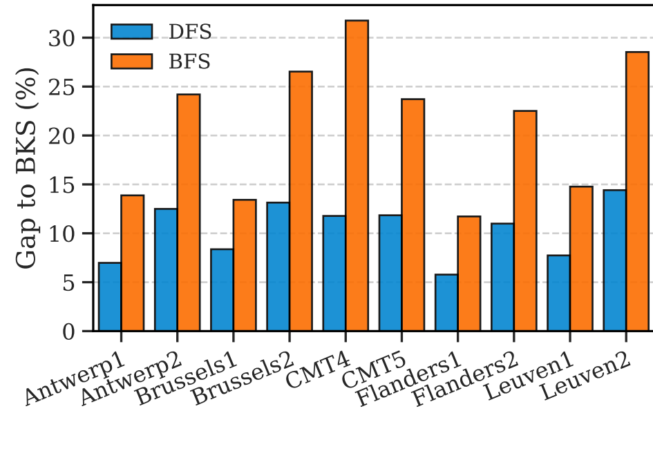
(c) Gap to BKS(%): DFS vs. BFS
