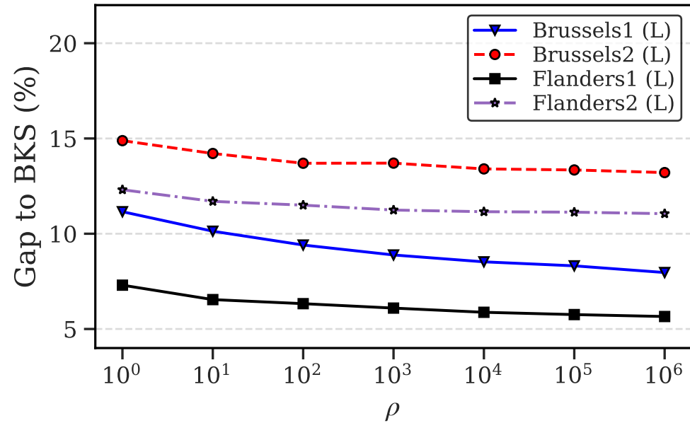
(a) Gap vs. \rho
