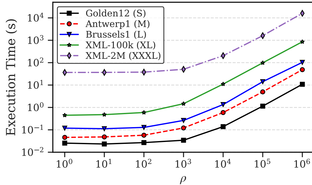
(b) Execution Time vs. \rho
