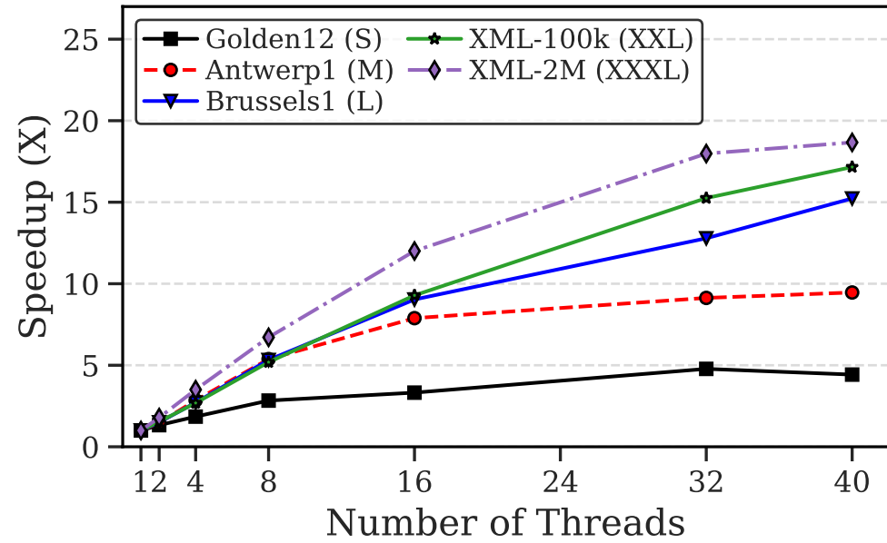
(c) Speedup vs. Threads
