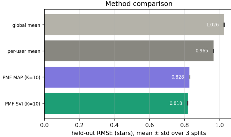
Figure 3: Method comparison at K=10 (mean \pm std over 3 splits). Both factorization models beat the mean baselines; SVI beats MAP on every split.
