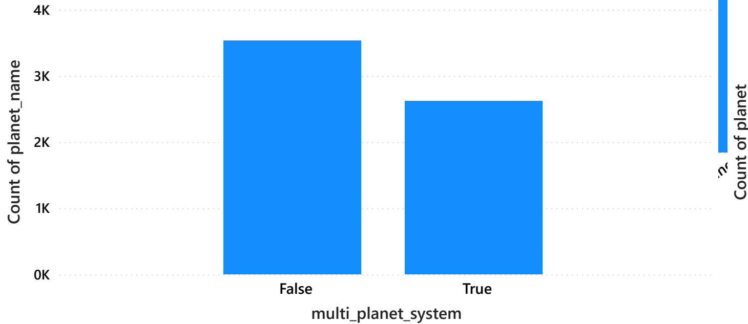
Count of planet_name by multi_planet_system
