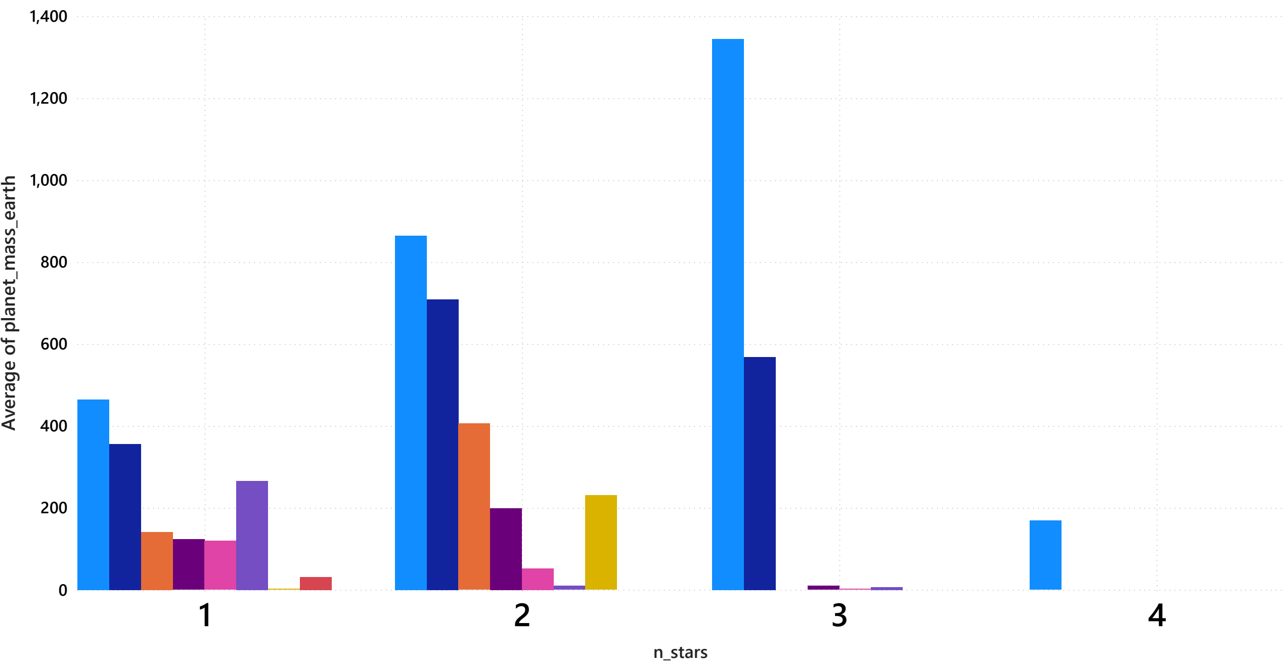
Average of planet_mass_earth by n_stars and n_planets
