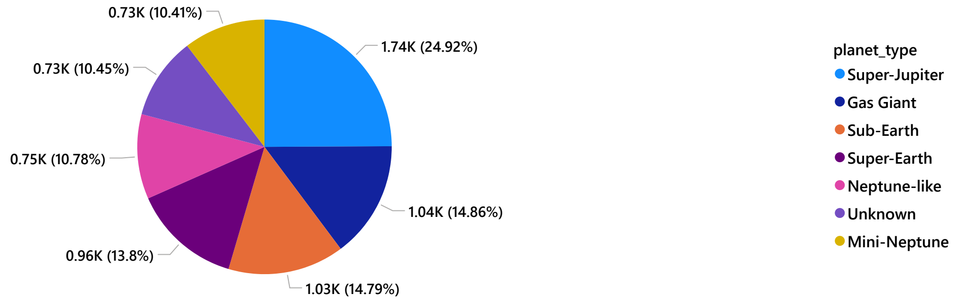
Average of equilibrium_temp_k by planet_type
