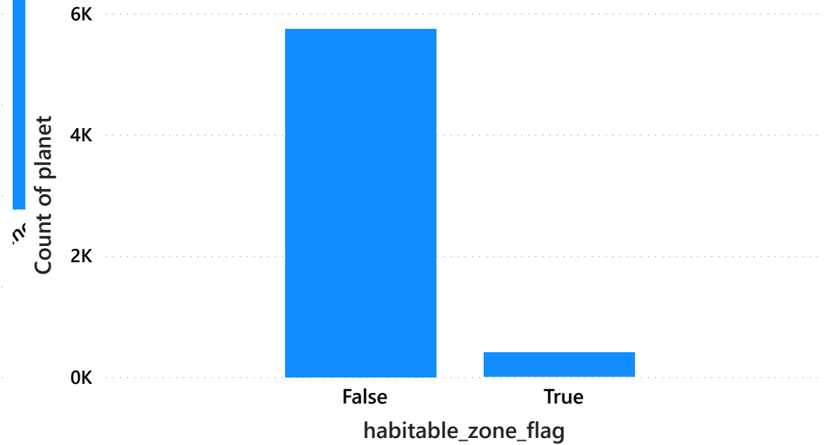
Count of planet_type by habitable_zone_flag
