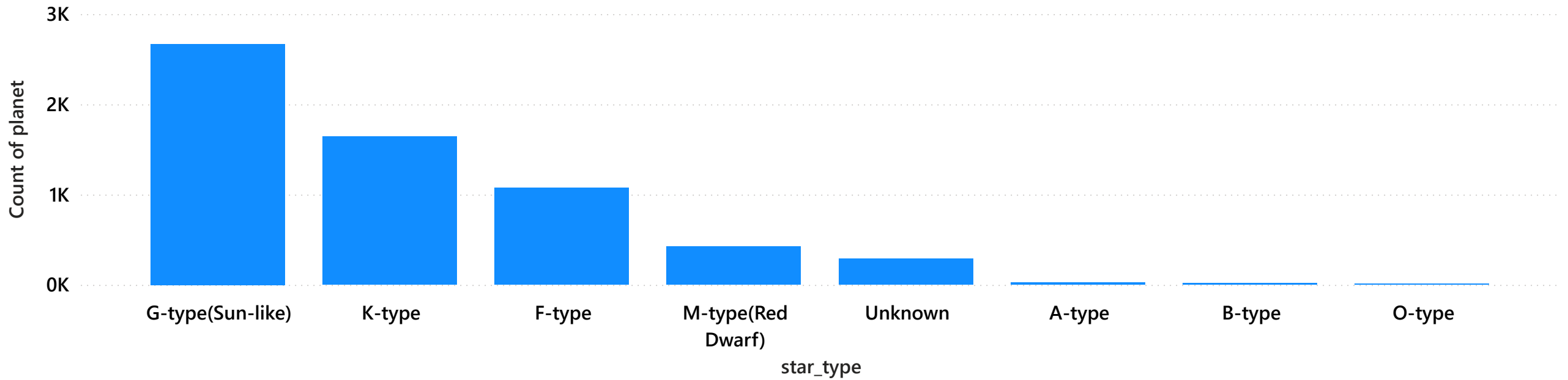
Count of planet_name by star_type
