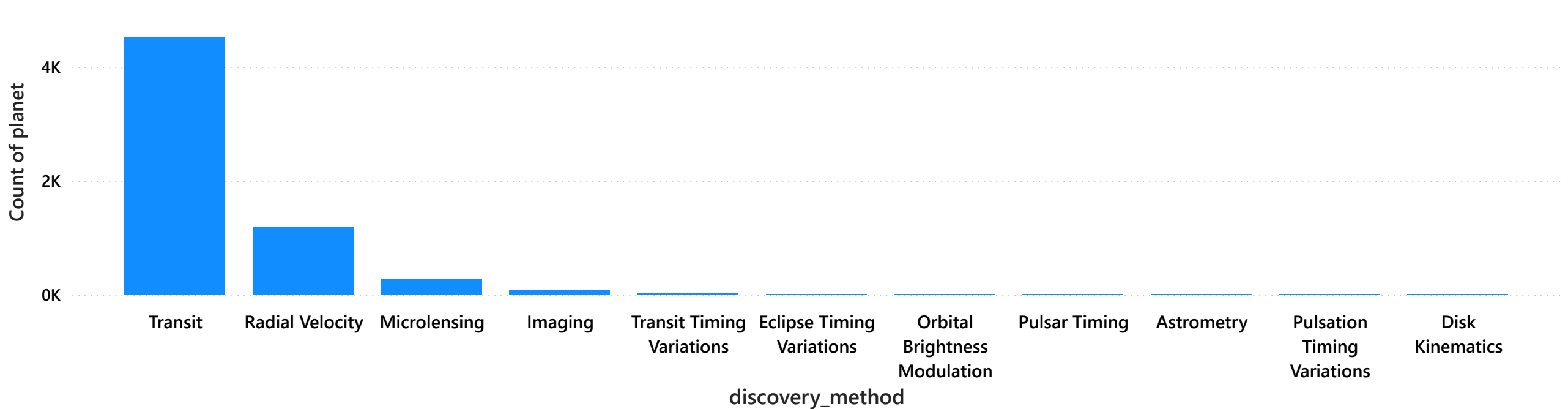
Count of planet_name by discovery_method
