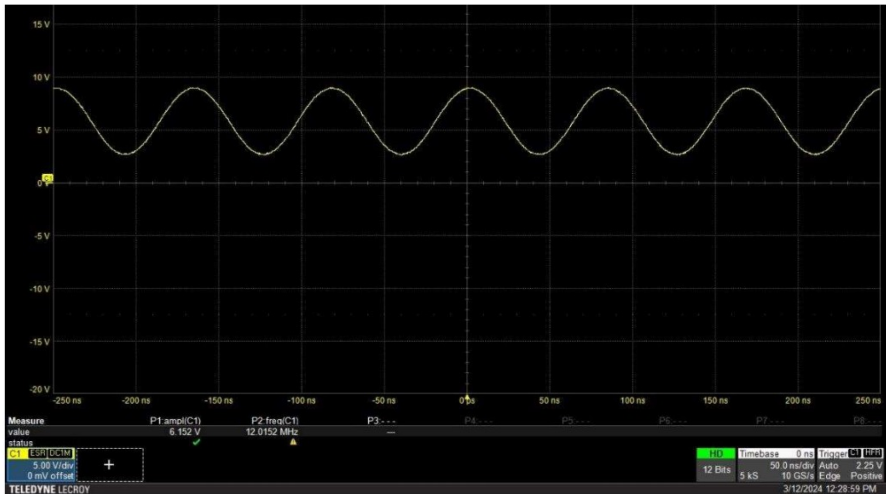
Picture 15: Quartz Oscillator, 13 V Vcc
