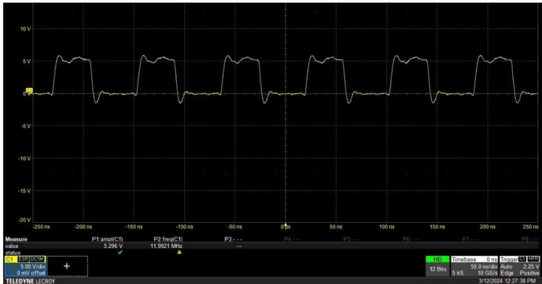
Picture 16: Quartz Oscillator, with 74HC00 5V Vcc
