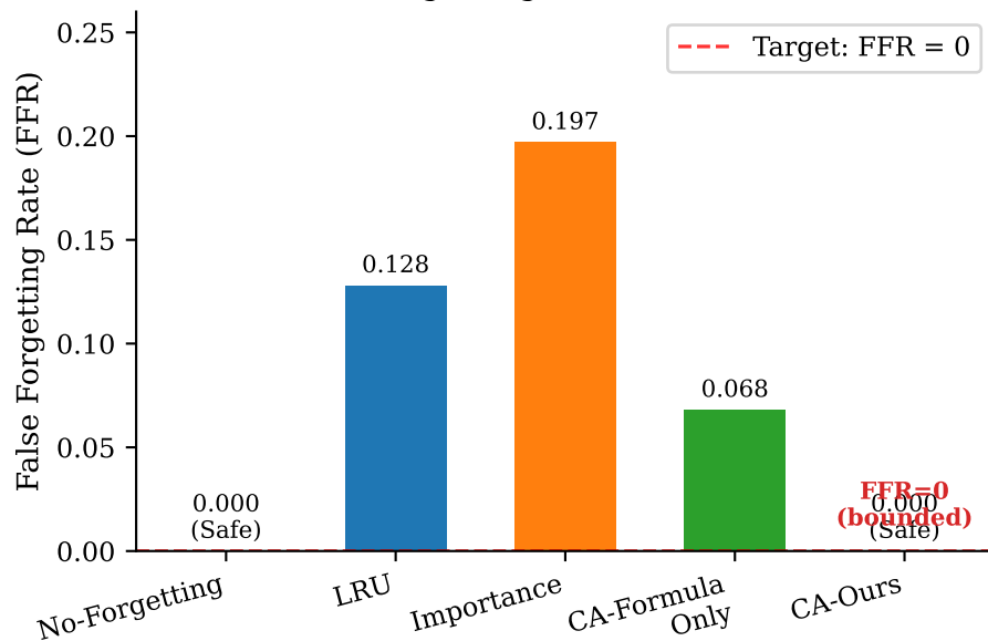
(b) False Forgetting Rate (FFR \downarrow is better)
