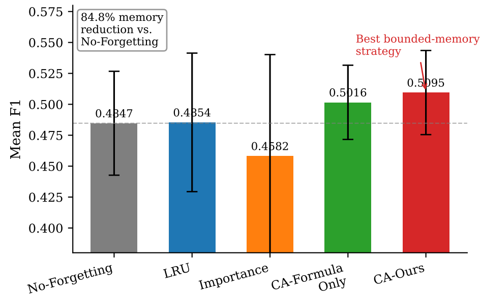
(a) Mean F1 Across 5 Runs
