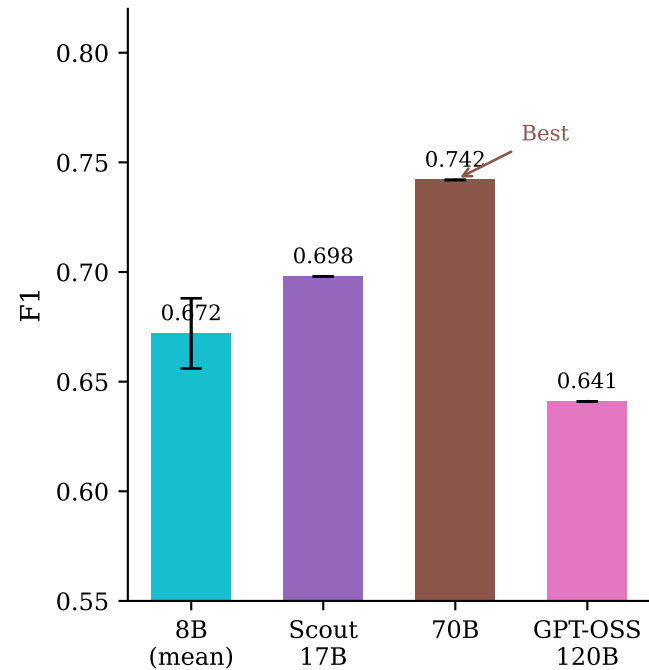
(a) F1 by Model
