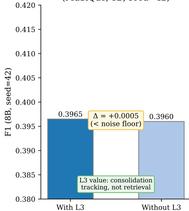
(c) L3 Knowledge Graph Ablation (MuSiQue, 8B, seed=42)
