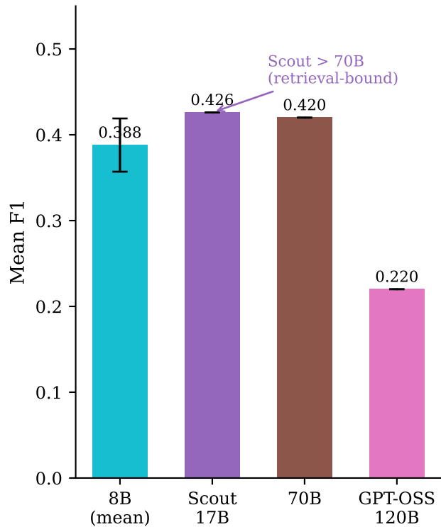
(a) Overall F1 (100 Questions)
