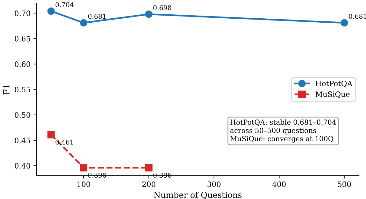
Figure 8: F1 Stability vs. Question Count (Llama 3.1 8B, seed=42)
