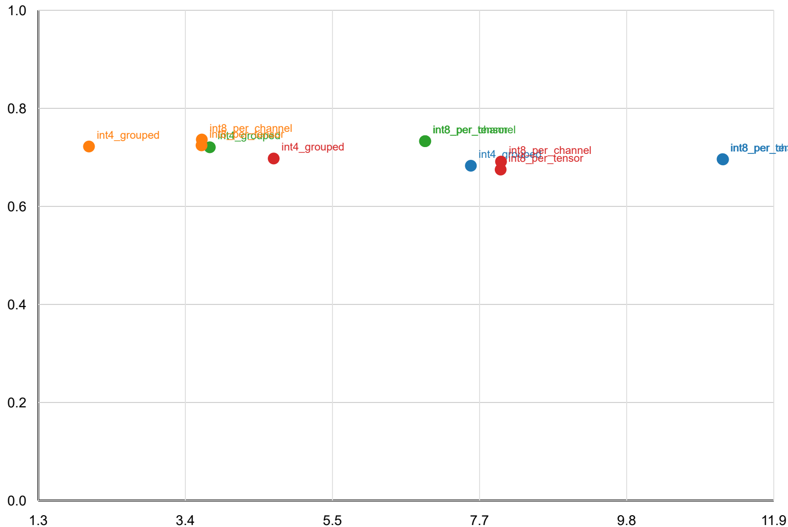
HELLASWAG quantized size vs accuracy
