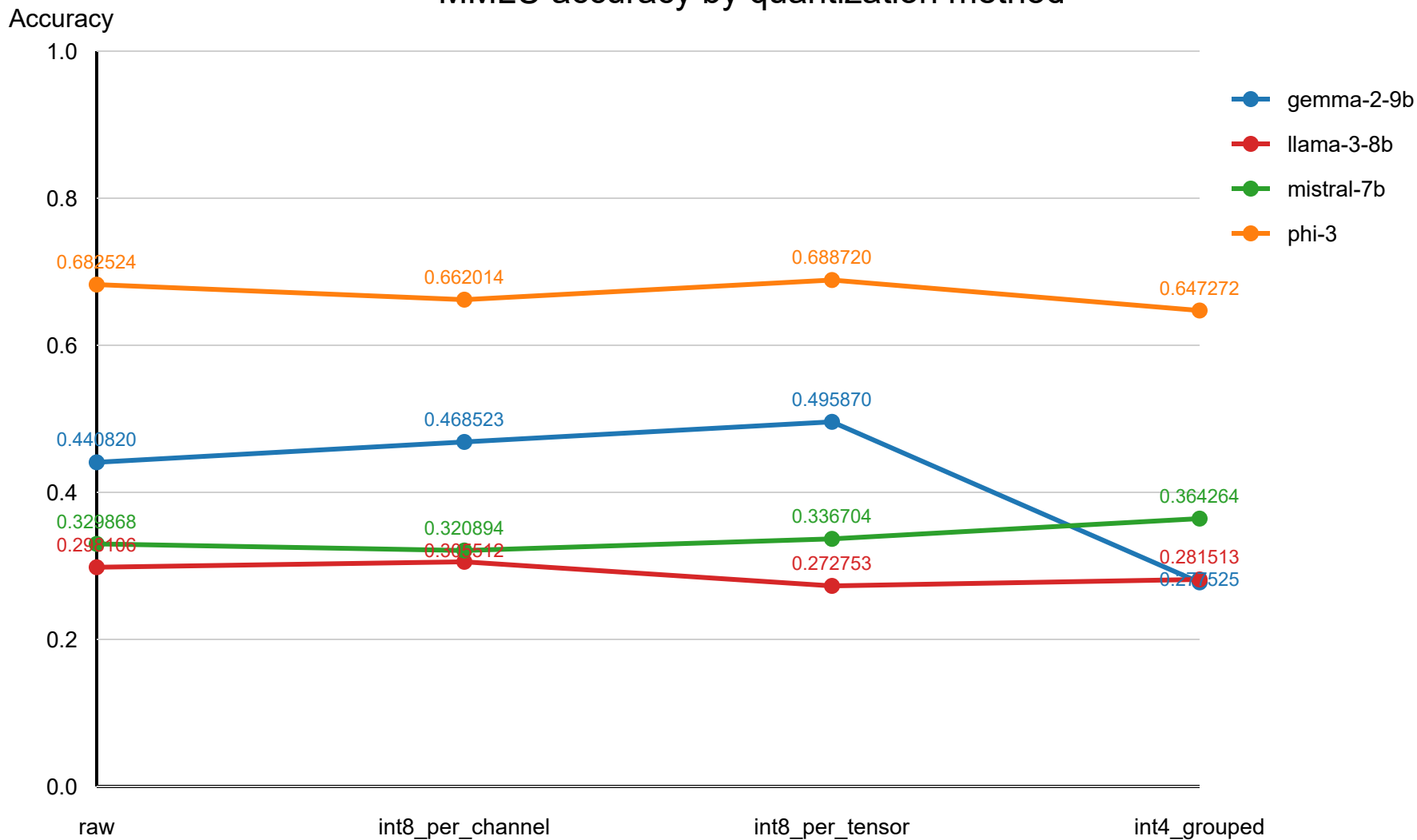
MMLU accuracy by quantization method
