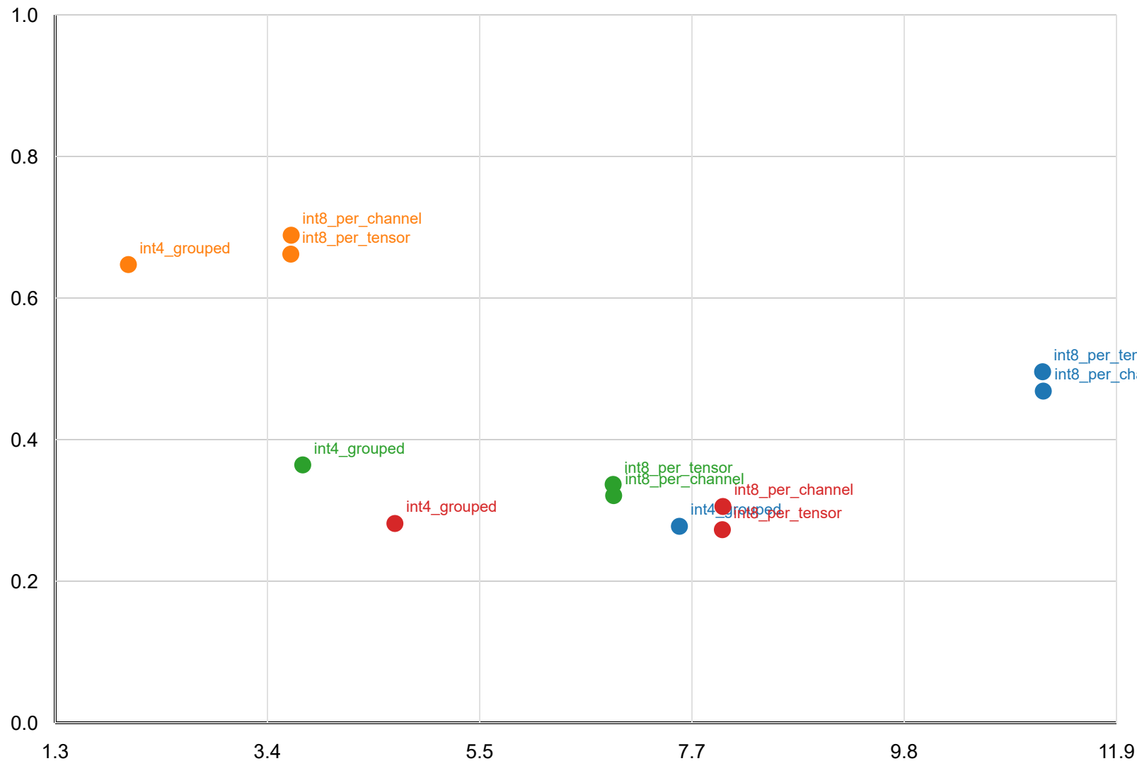
MMLU quantized size vs accuracy
