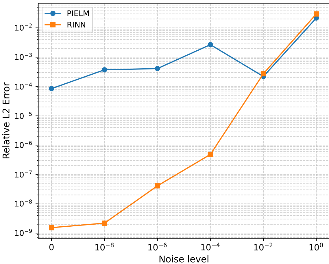
Relative L2 Error vs Noise Level
