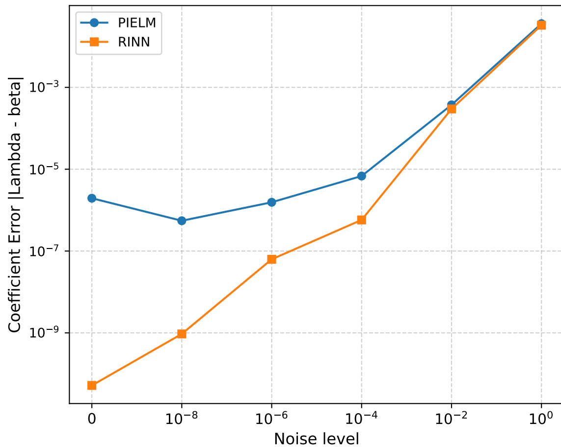
Coefficient Error vs Noise Level
