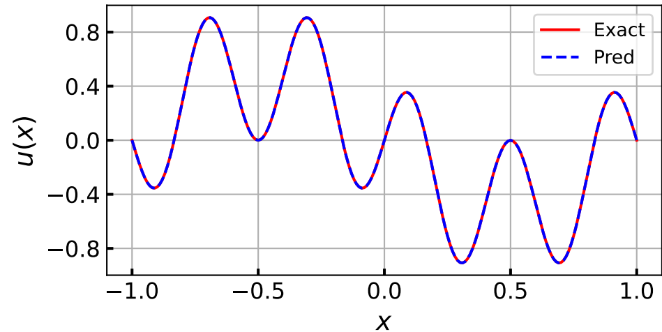
Exact & Numerical
