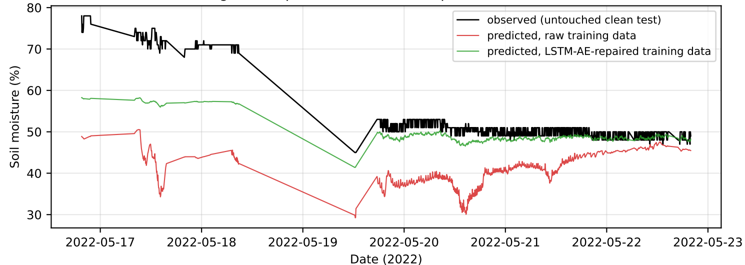
Effect of training-data repair on common-test predictions (seed 42, real data)
