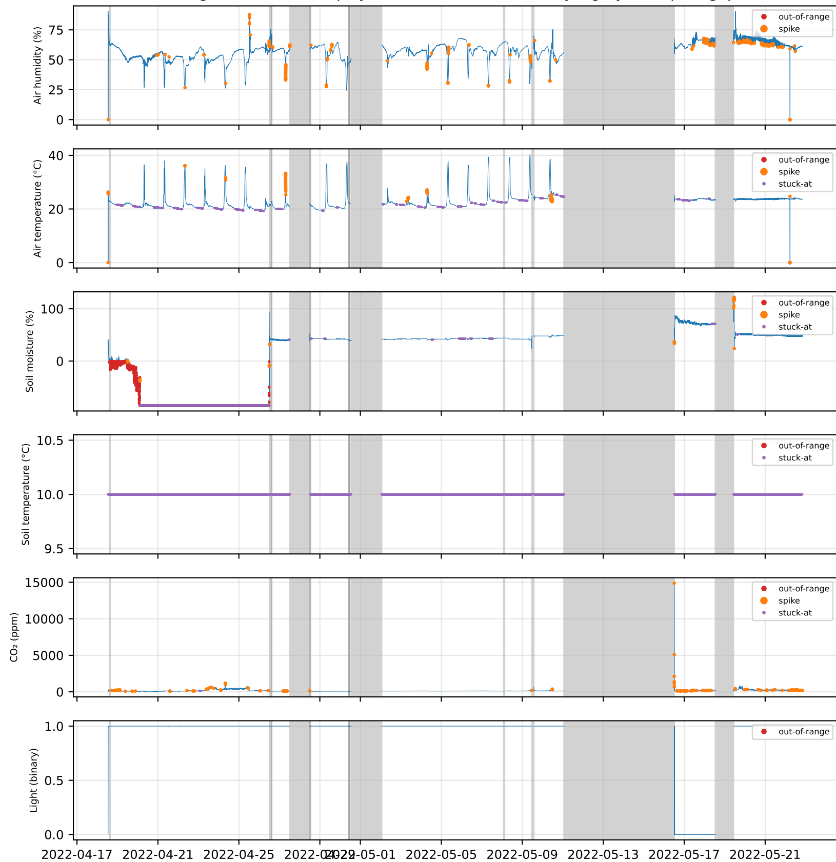
Raw greenhouse IoT deployment with real fault overlays (gray = dropout gaps)
