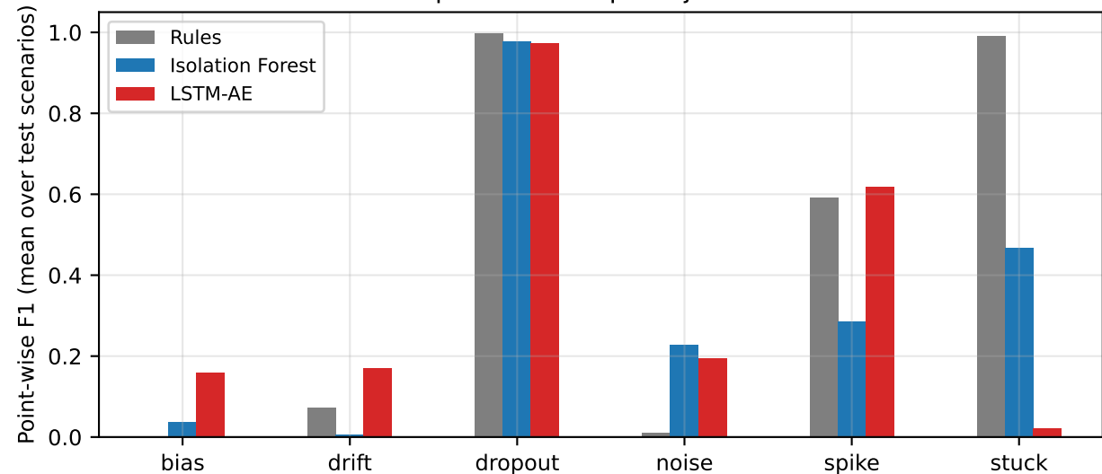
Detection performance per injected fault class
