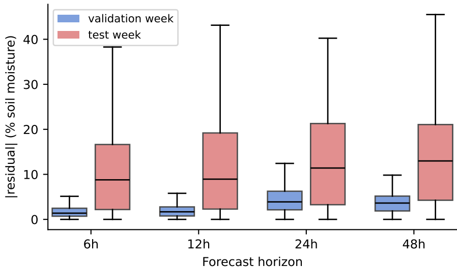
LSTM absolute residuals: validation vs. test (20 seeds pooled)
