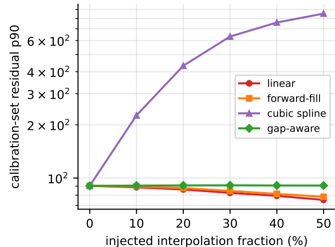
(a) residual-scale distortion
