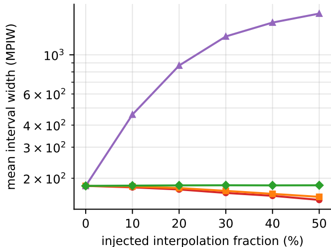
(b) resulting interval width
