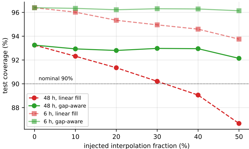
USCRN Fairhope replication (persistence SCP)
