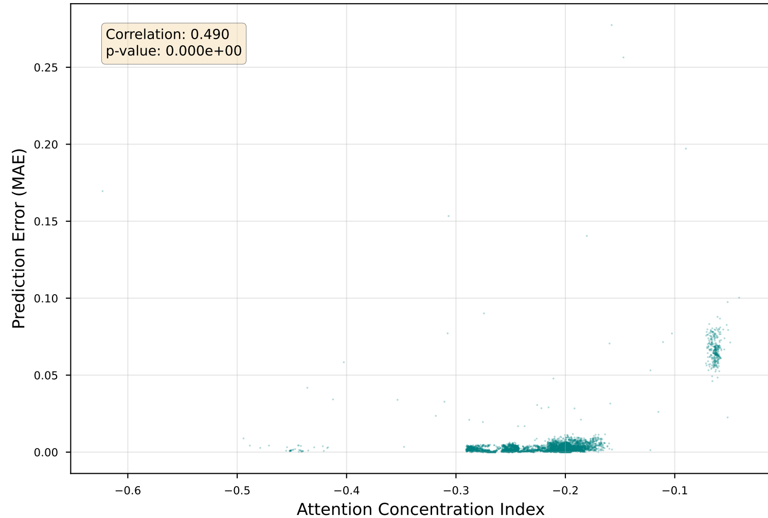
Attention Concentration vs Prediction Error (20,000 samples)
