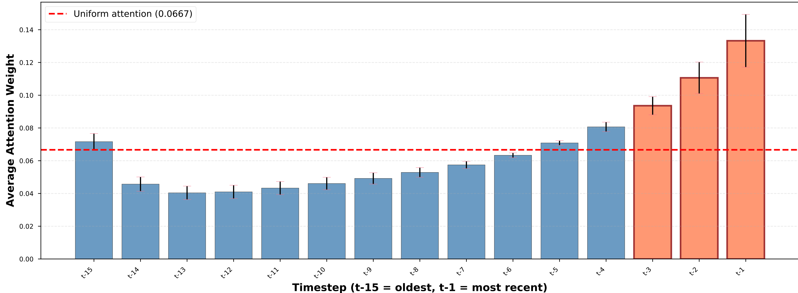
Average Attention Distribution Across Timesteps (Error bars show standard deviation)
