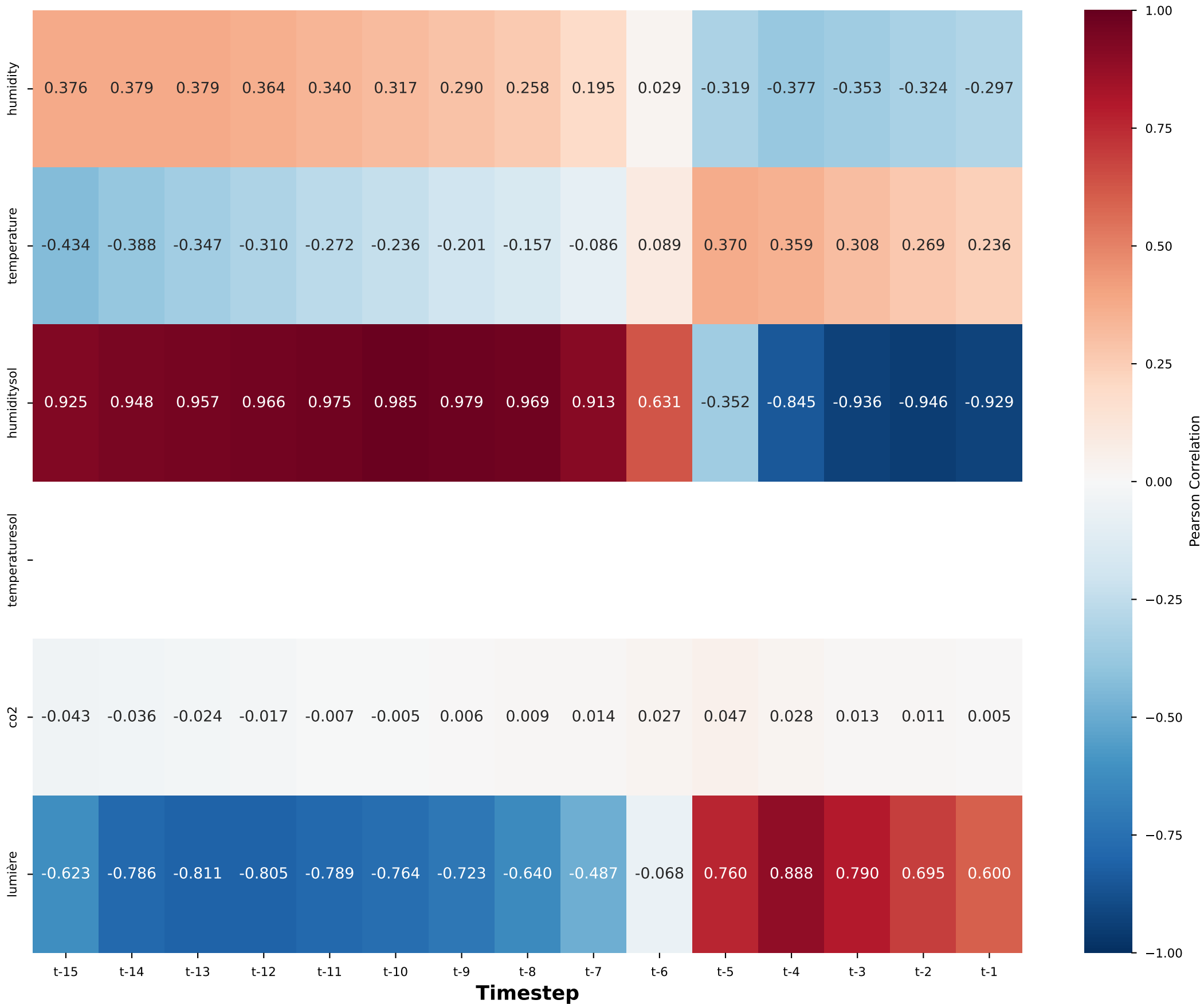
Feature Value vs Attention Weight Correlation (Based on 5,000 samples)
