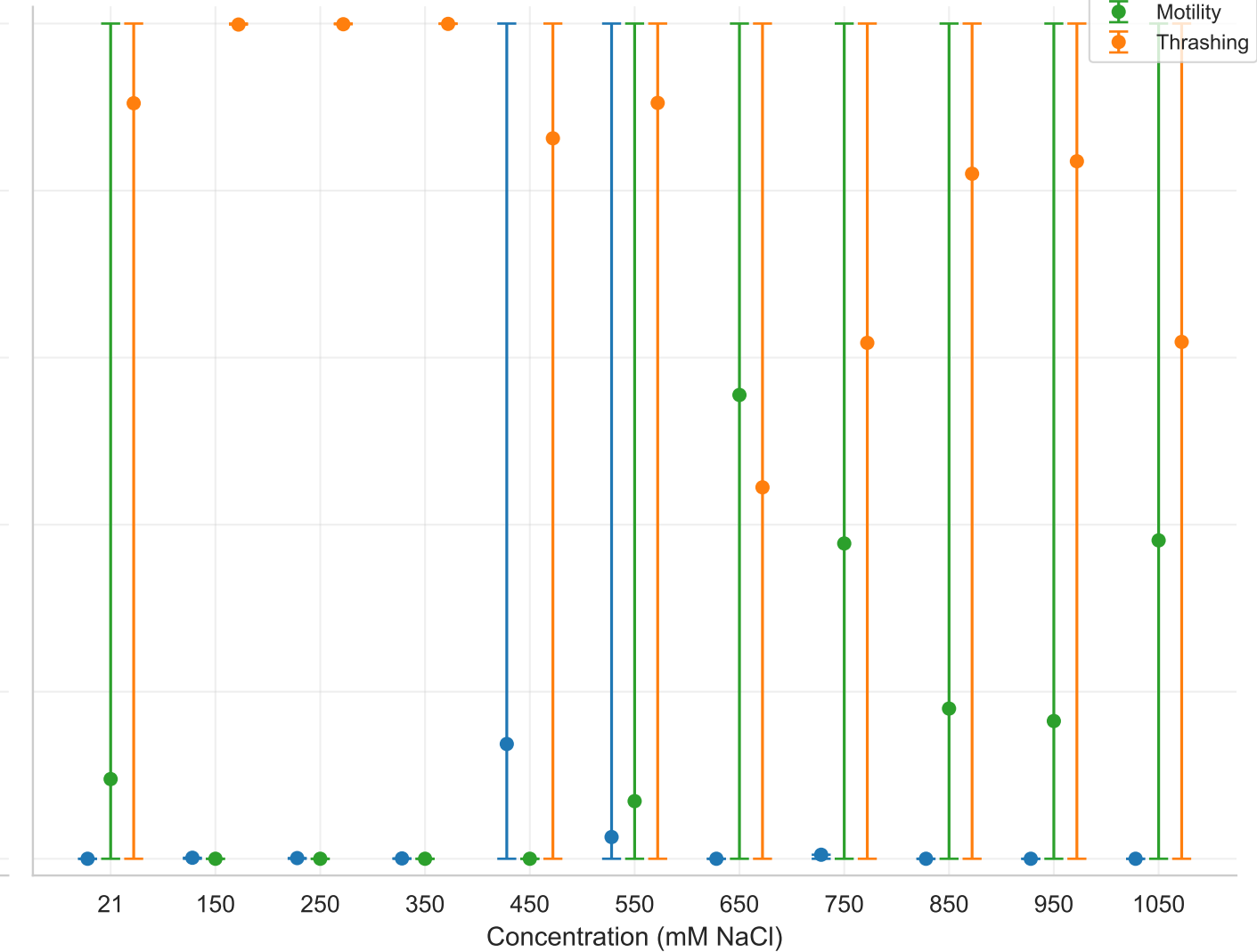
Earliest-Event Probability (25% threshold)
