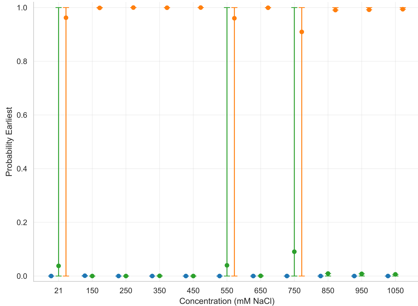
Earliest-Event Probability (50% threshold)
