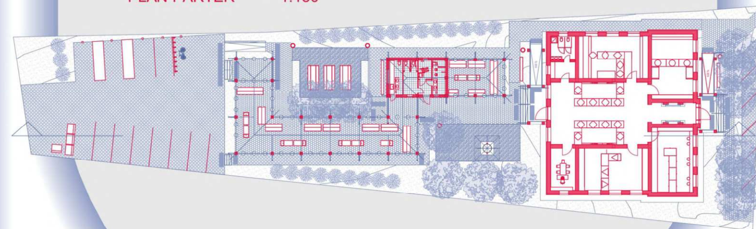
PLAN PARTER 1:150
