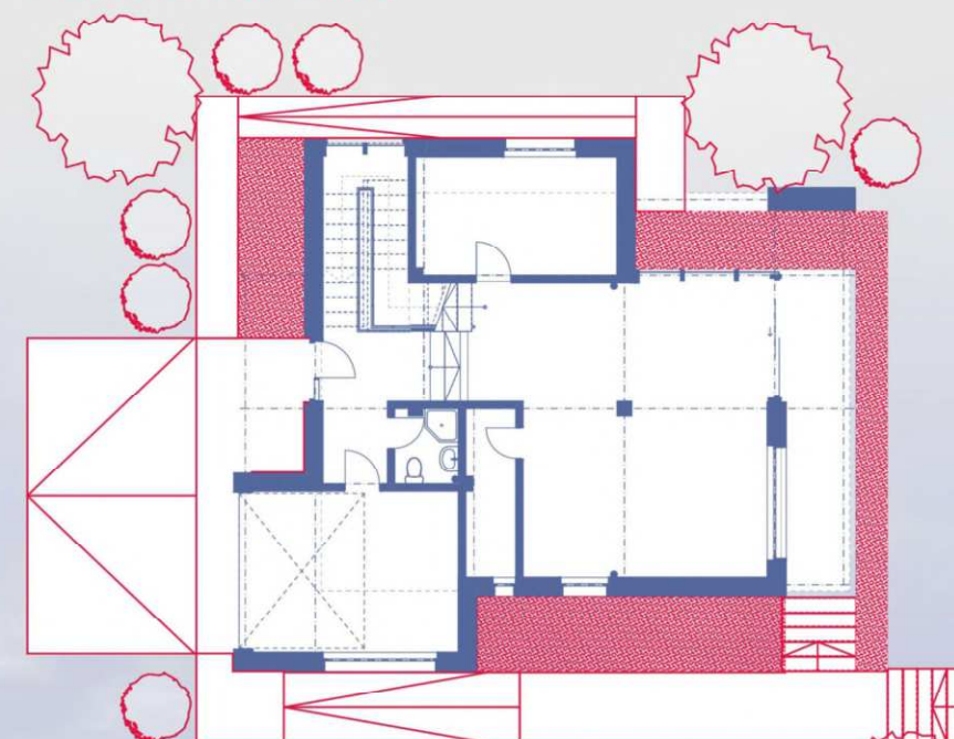
PLAN PARTER 1:100
