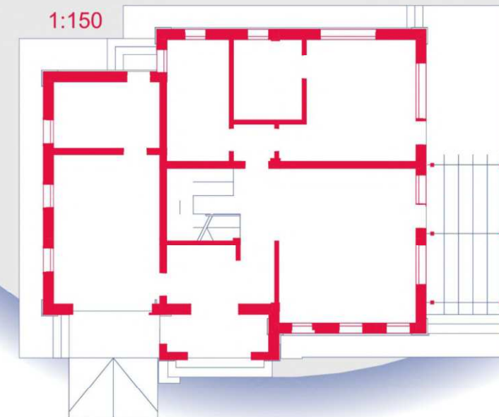
PLAN PARTER 1:150
