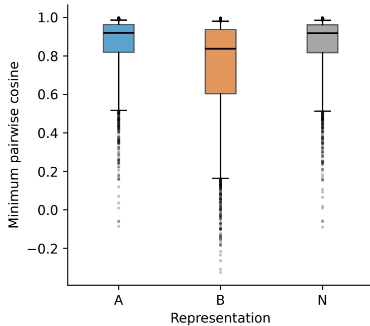
Augmentation stability: 2,502 BGCs (five states each)
