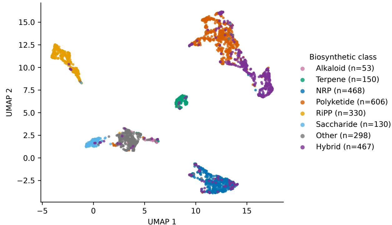
Biosynthetic classes of 2,502 consensus BGCs
