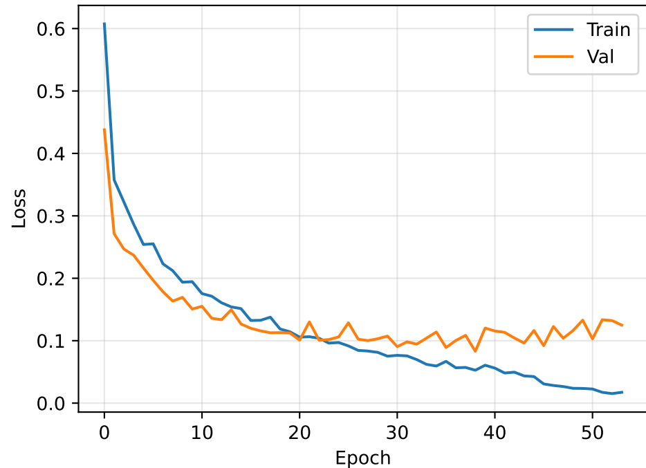
Loss Curve
