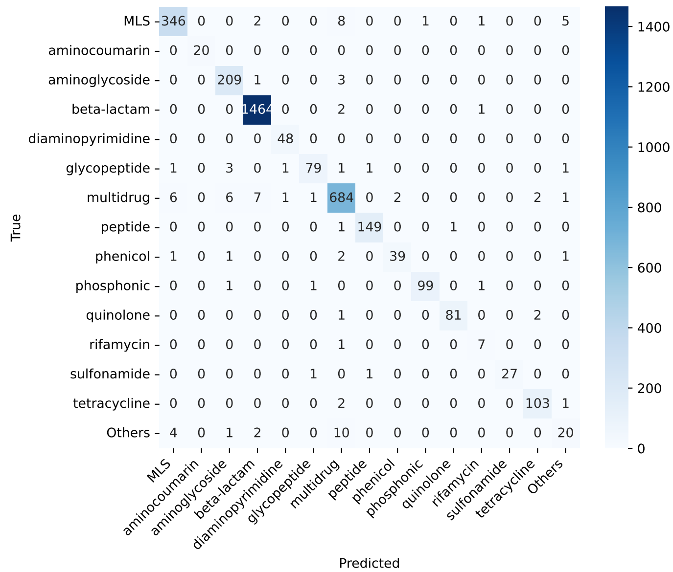
Confusion Matrix
