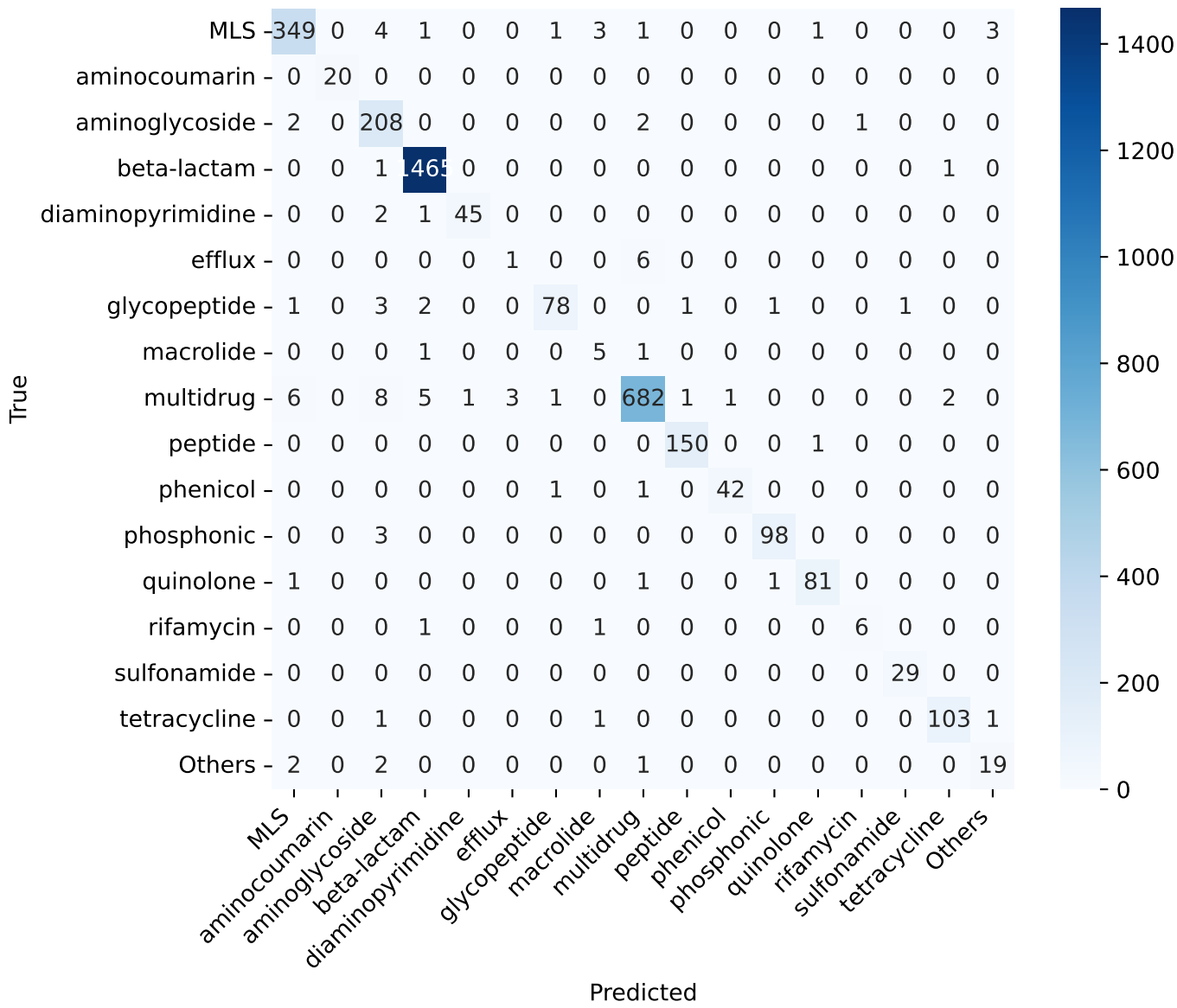
Confusion Matrix
