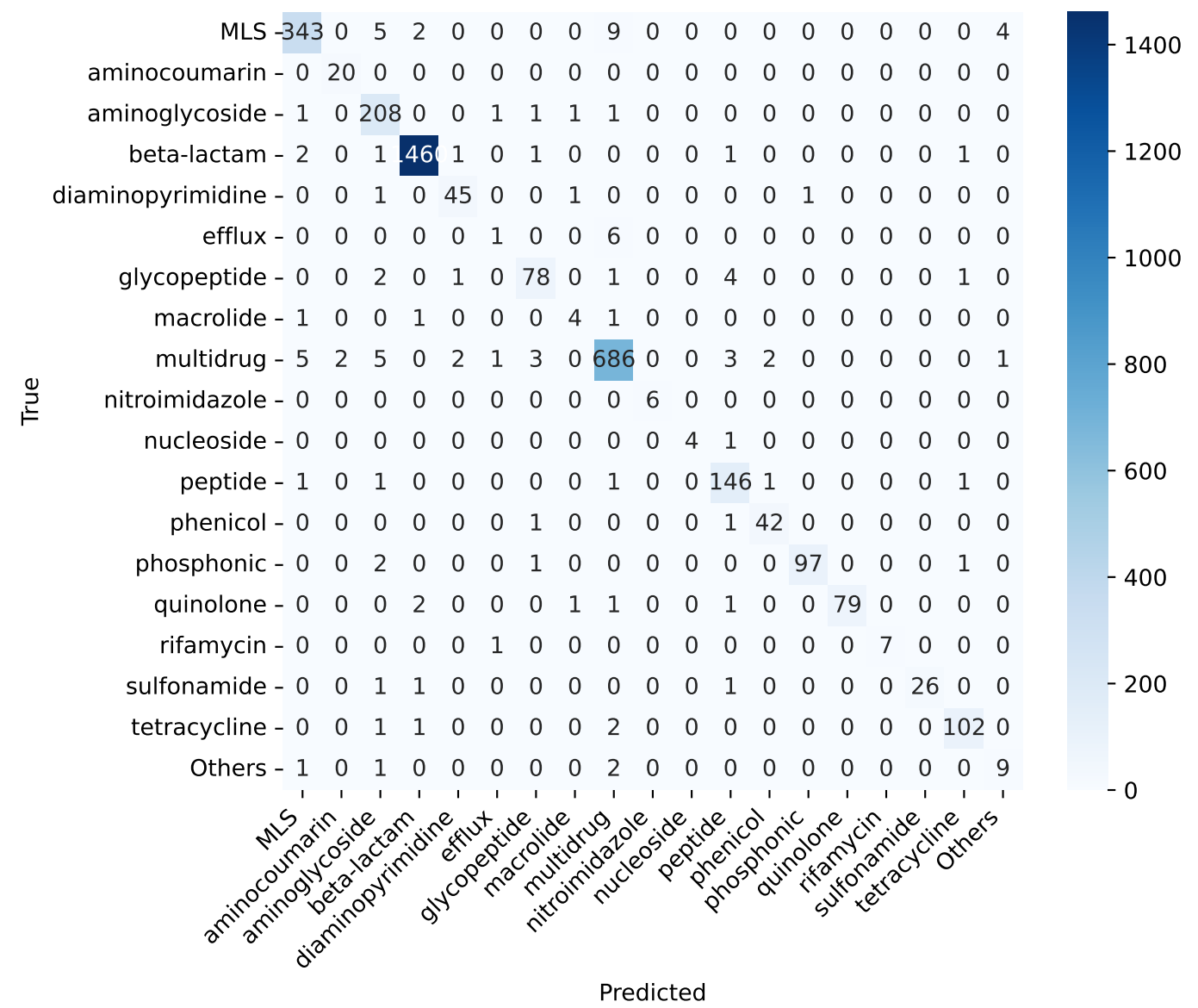
Confusion Matrix
