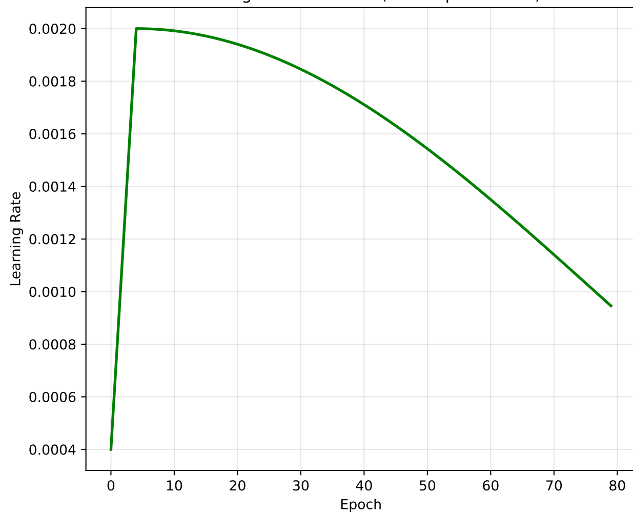
Learning Rate Schedule (Warmup + Cosine)
