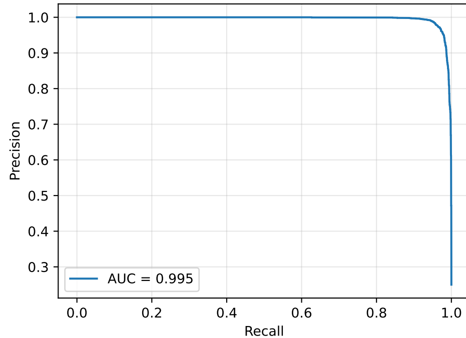
PR Curve
