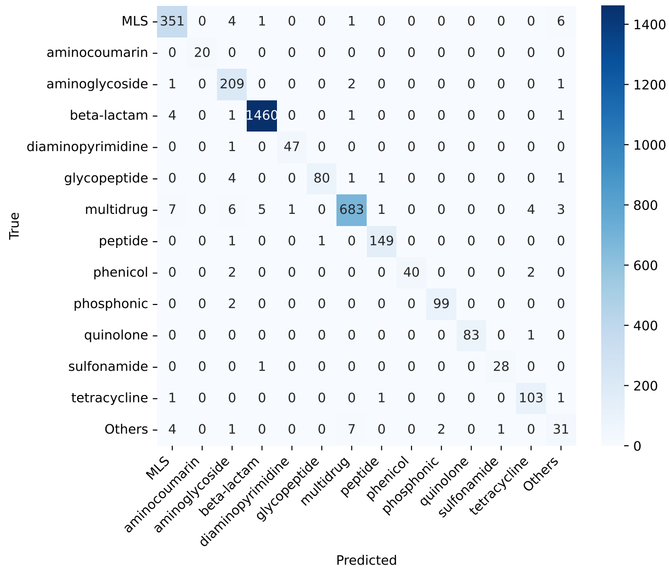
Confusion Matrix
