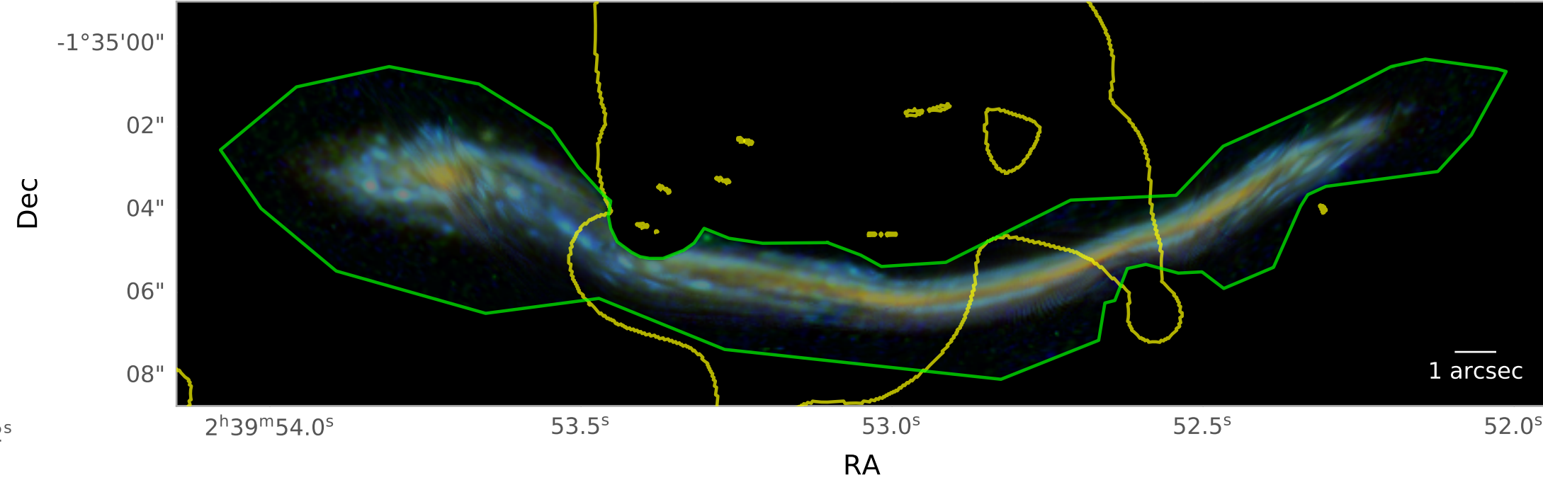
Re-Lensed Re-Convolved RGB Optimized Model Arc
