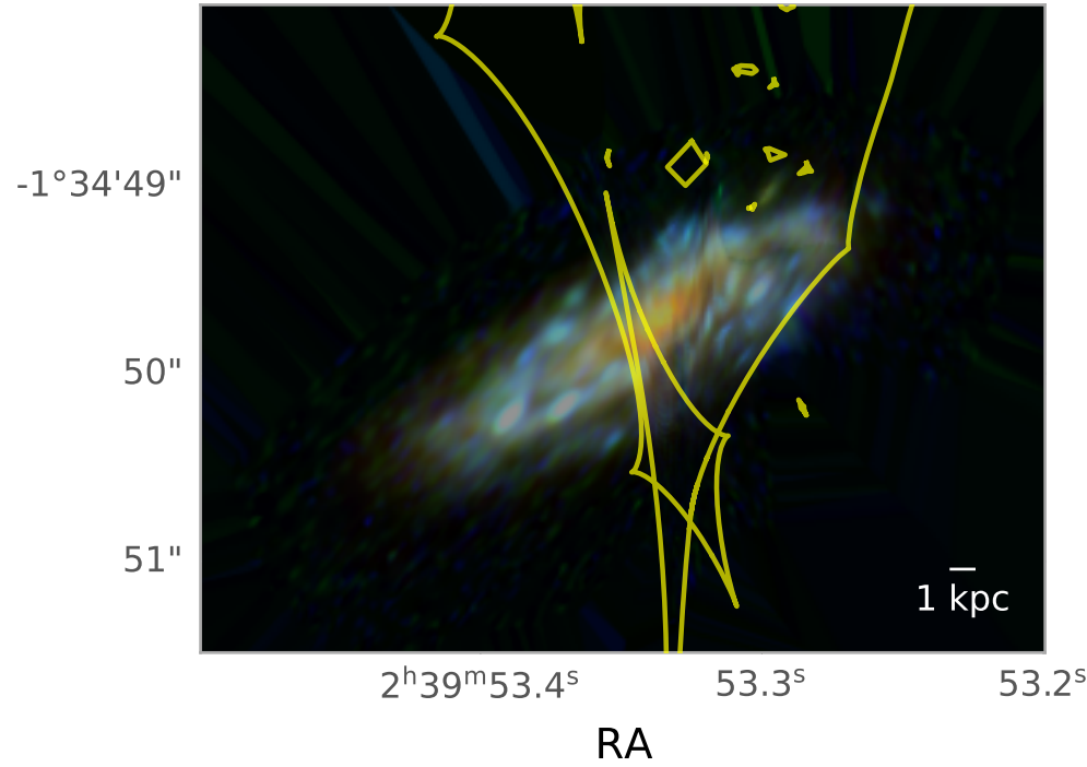
Reconstructed Source Model De-Lensed and Smoothed
