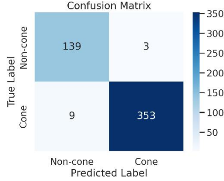
Fig. 2. Confusion Matrix on Test Split
