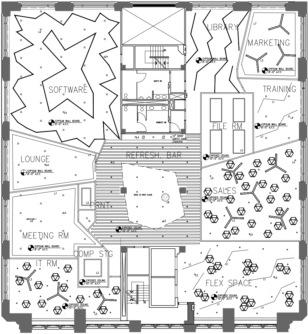
Second Floor Reflected Ceiling Plan Scale: 1/8" - 1'0"
