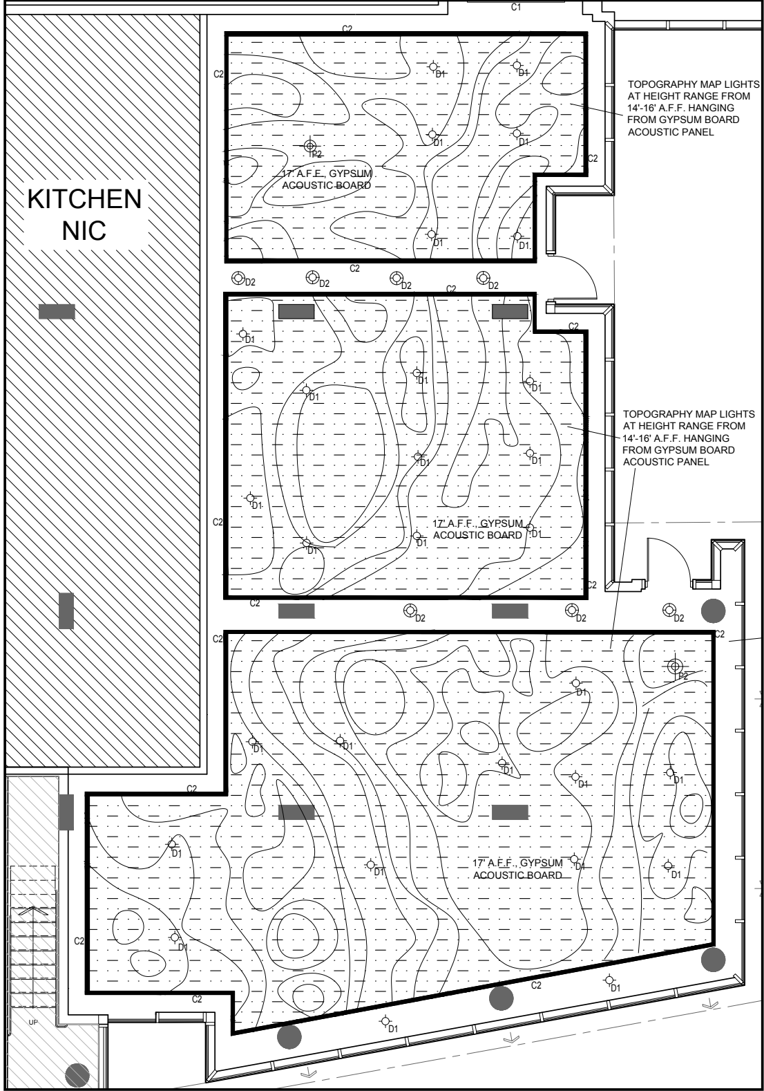
Reflected Ceiling Plan Scale: 1:50
