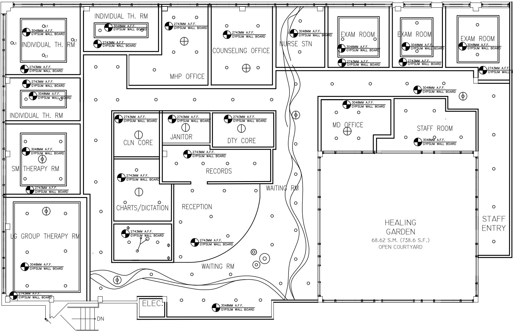
Reflected Ceiling Plan Scale: NTS
