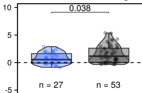
Cat. residues/DHF binding
