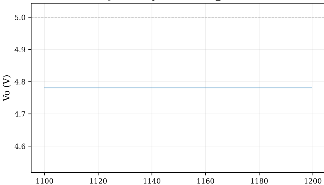
Output Voltage — CCM ( R_{load}=5\Omega )
