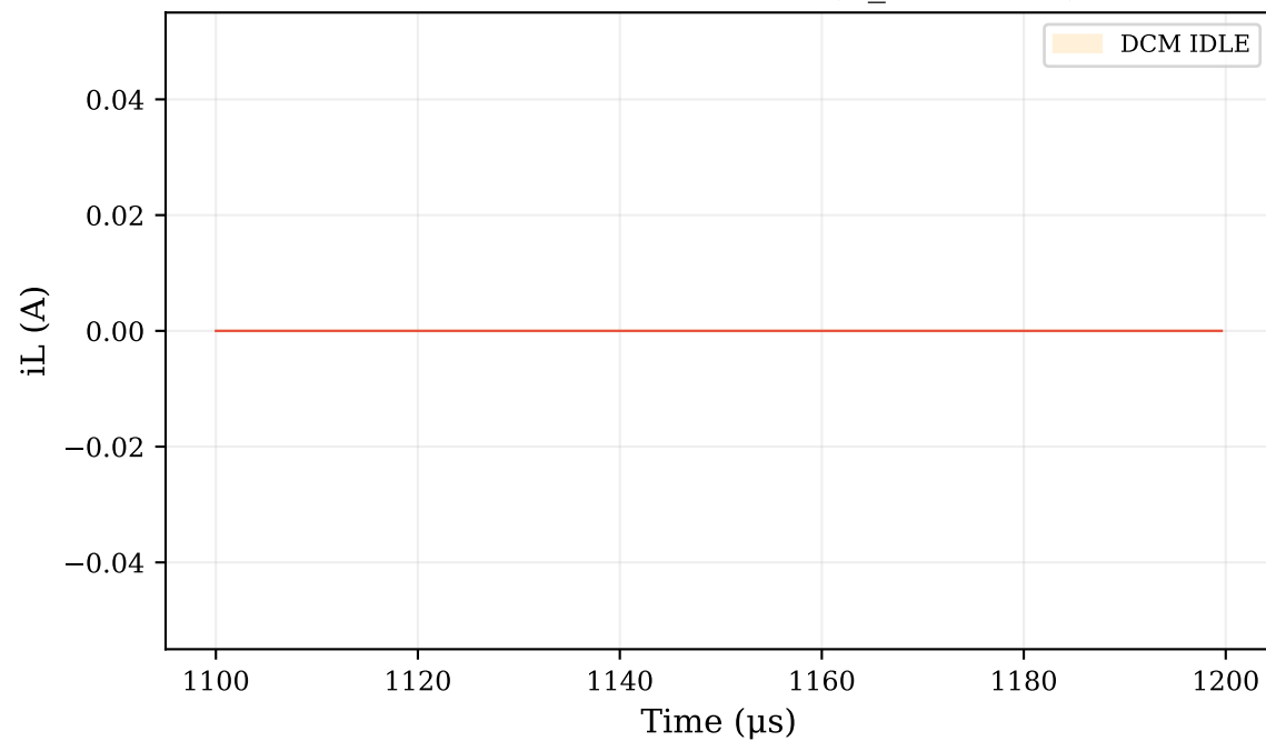
Inductor Current — DCM ( R_{load}=50\Omega )
