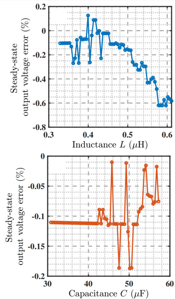
(b) Steady-state output voltage error vs L/C
