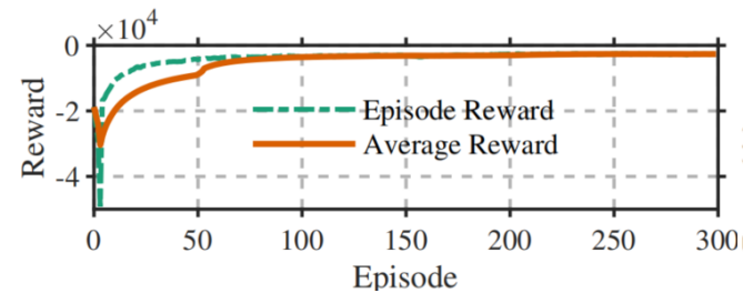
(a) Reward Curve
