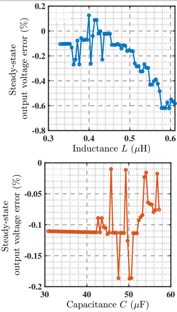
(b) Steady-state output voltage error vs L/C
