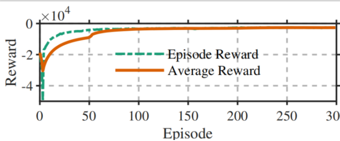
(a) Reward Curve
