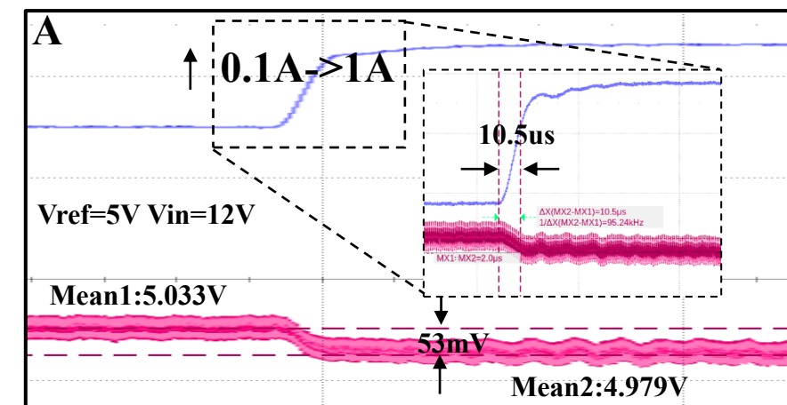
(f) Dynamic Response Performance
