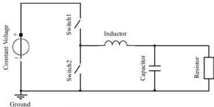
(a). Buck topology.
