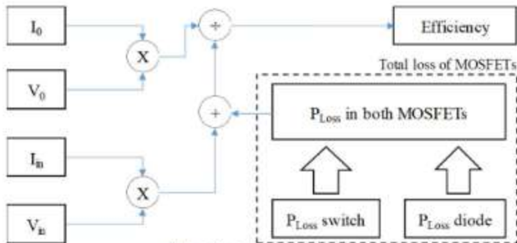
(b). Efficiency calculation.
