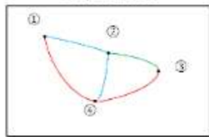
Graph Dataset
