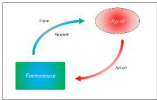
Reinforcement learning
