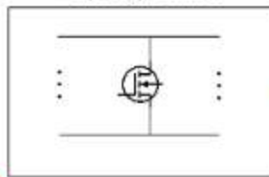
Topology Dataset
